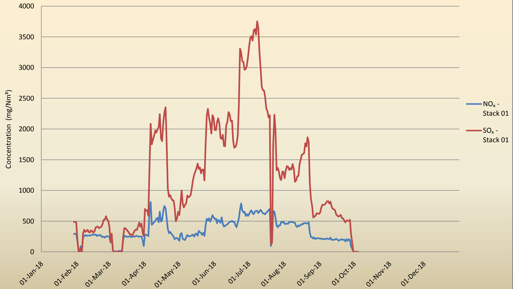
Annual Emission Trend of Gaseous in M/s. Vardhaman Yarns, Dist. Raisen (M.P.)
